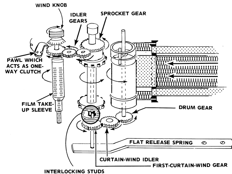
FIGURE 28 ARROWS INDICATE TRAVEL DIRECTIONS DURING WIND CYCLE
