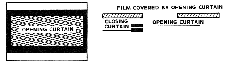
FIGURE 3 SHUTTER COCKED
