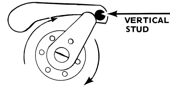
OPENING CURTAIN RELEASED, CLOSING-CURTAIN CAM HELD BY CLOSING-CURTAIN LATCH (ARROWS INDICATE ROTATION ON RELEASE CYCLE)
