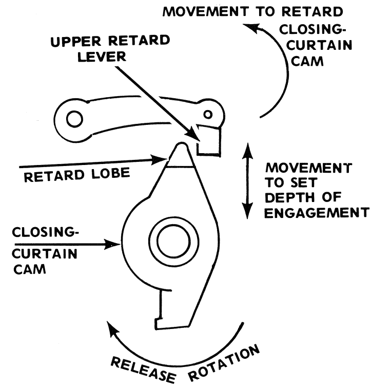
FIGURE 52
