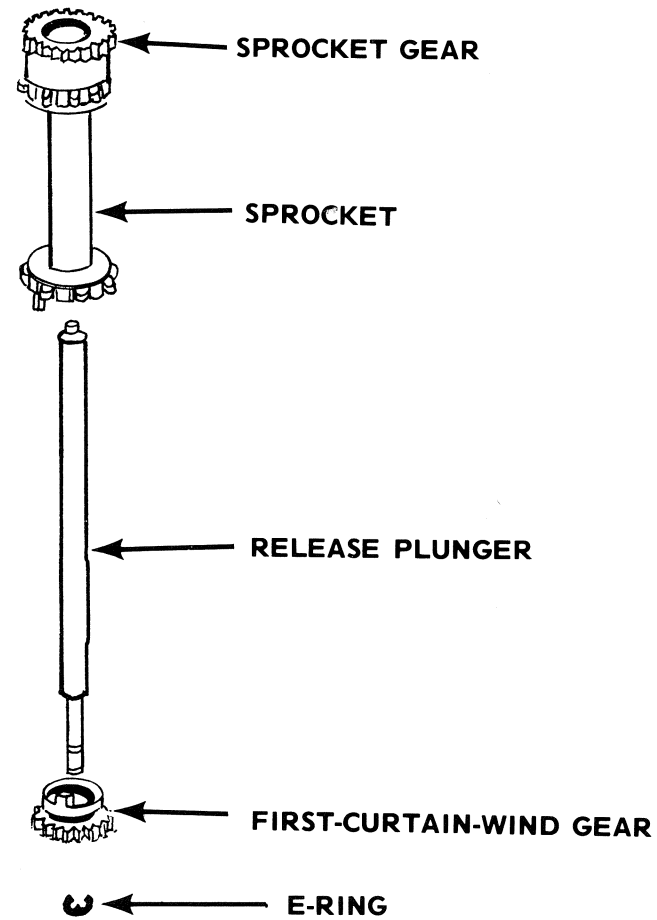
FIGURE 29 SPROCKET AND RELEASE PLUNGER
