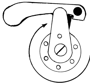
FIGURE 45 OPENING CURTAIN RELEASED ON "BULB" — DISENGAGING LEVER CAN'T TRAVEL FAR ENOUGH TO REACH CLOSING-CURTAIN LATCH
