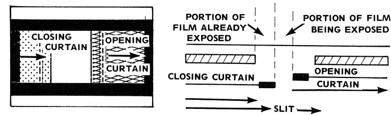
FIGURE 5 CLOSING CURTAIN FREED
