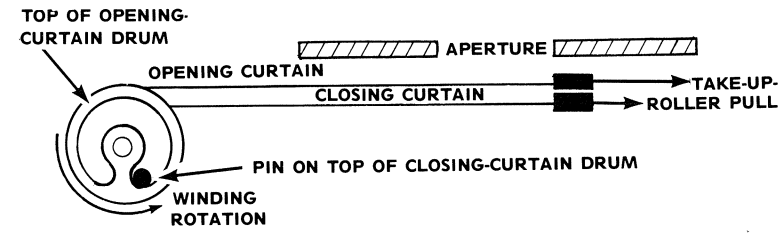
FIGURE 24 RELEASED POSITION
