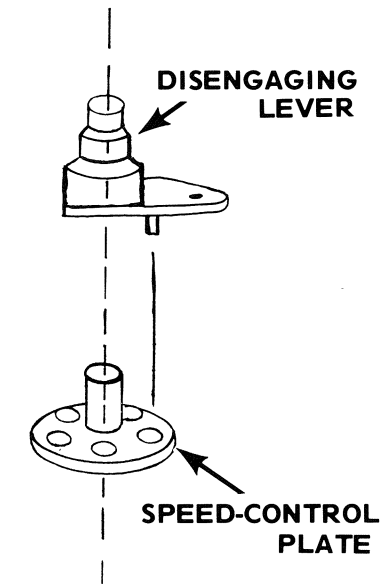
FIGURE 39
