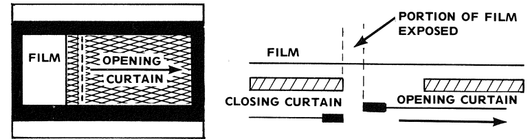
FIGURE 4 OPENING CURTAIN RELEASED
