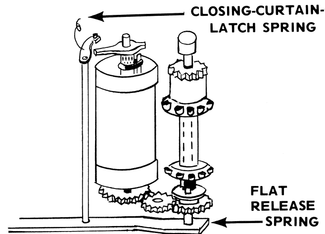
FIGURE 33 FROM BACK OF SHUTTER
