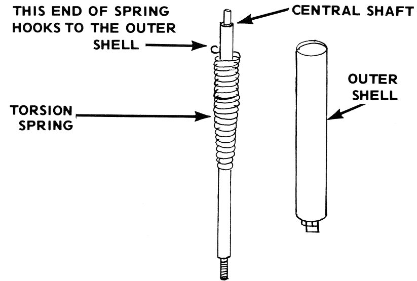
DESIGN OF CLOSING-CURTAIN TAKE-UP ROLLER FIGURE 15
