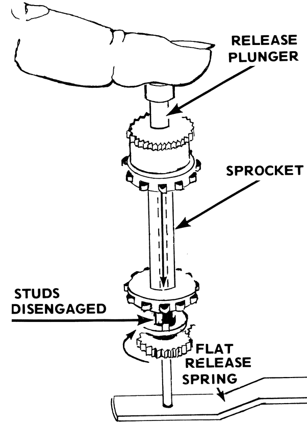
FIGURE 30 FIRST CURTAIN WIND GEAR IS FREE TO ROTATE (IN DIRECTION OF ARROW)
