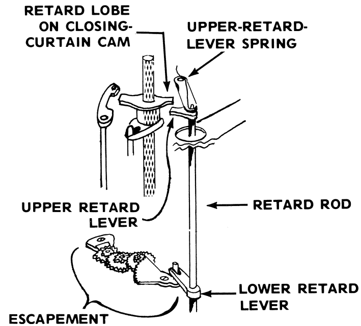
FIGURE 50
