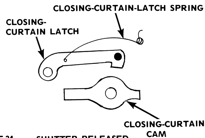
FIGURE 34 SHUTTER RELEASED
