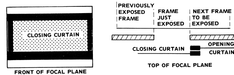
FIGURE 6 SHUTTER RELEASED
