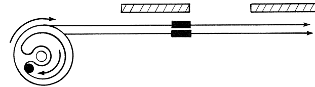
FIGURE 26 COCKED POSITION — ARROWS INDICATE DIRECTION OF PULL OF TAKE-UP-ROLLER SPRINGS
